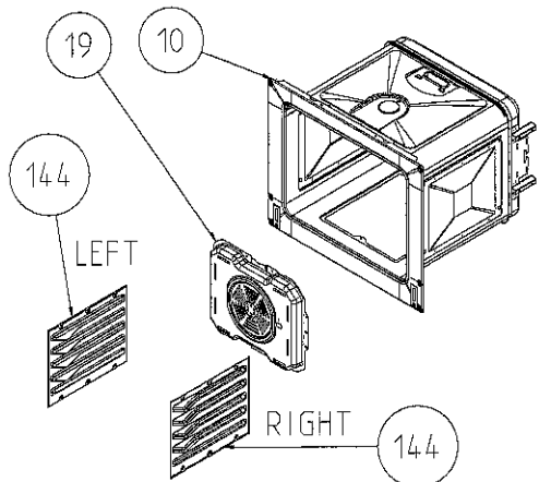
CAVITY ASSEMBLY WITH CATALYTIC SHELF ( OPTIONAL )
